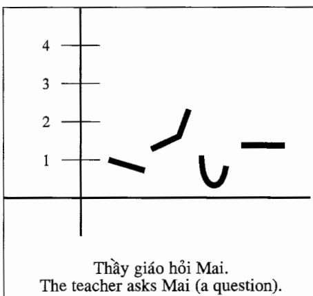
Figure 12: The intonation of an assertive sentence and an interrogative sentence.
