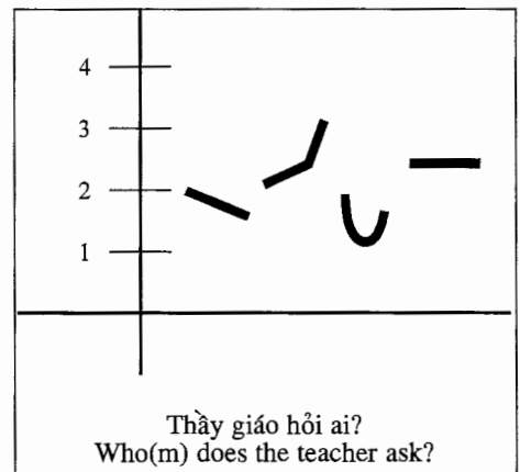
Figure 12: The intonation of an assertive sentence and an interrogative sentence.
