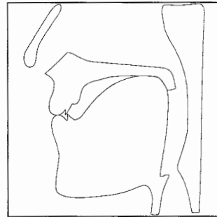
Figure 14: Tongue and lip position for the final ng after u, ô, o .
