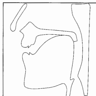
Figure 15: Tongue and lip position for the final nh after i , ê , e .
